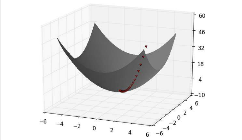
Figure 8-1. Finding a minimum using gradient descent
